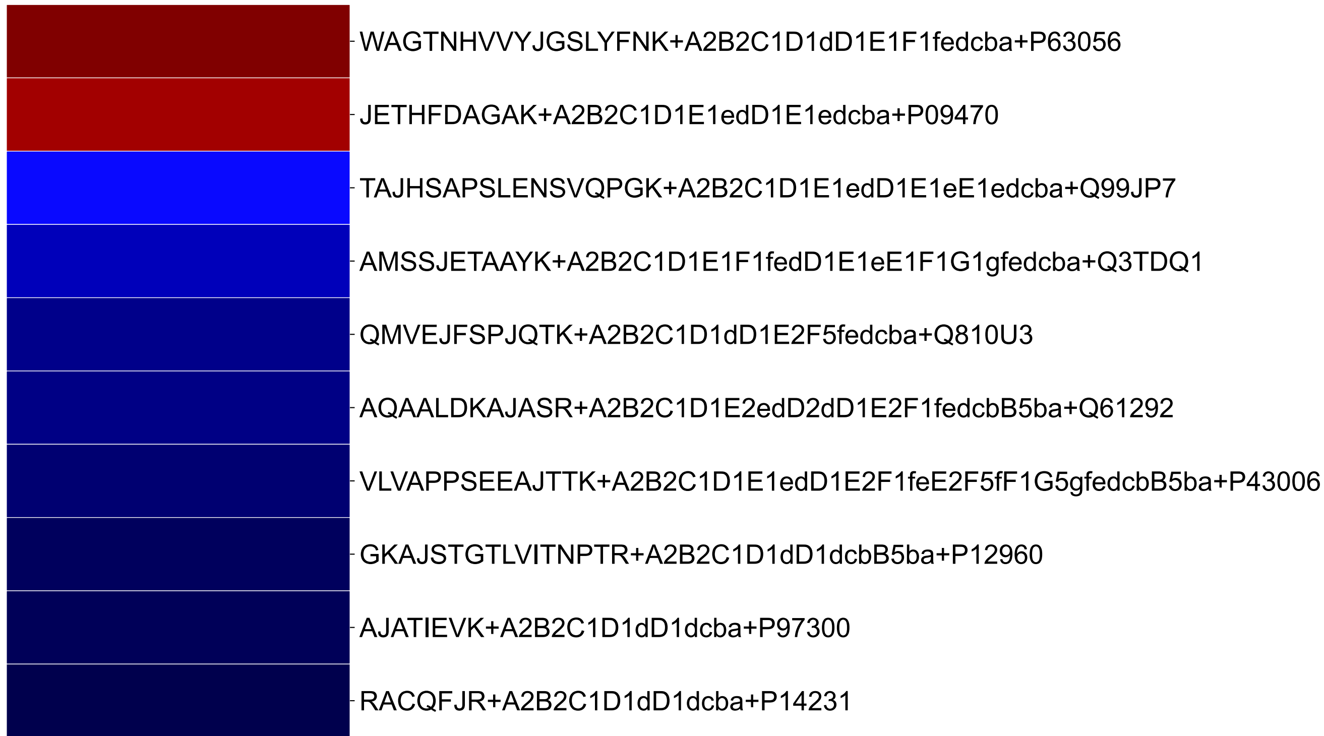
Random forest-based features importance score
